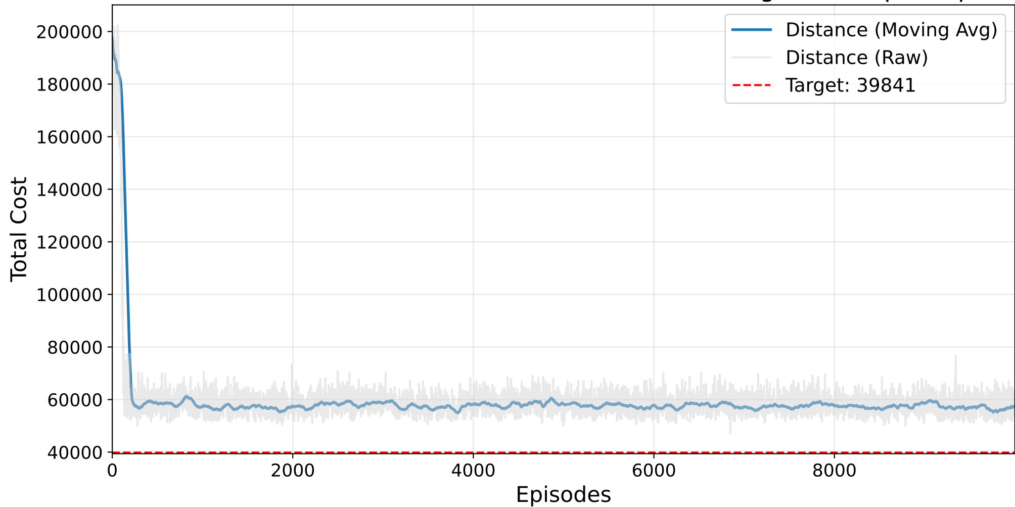
Final HYPERBAND TPE Masked AutoRL-SOP Training - kro124p.2.sop
